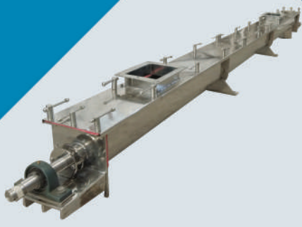
U Trough screw conveyor
